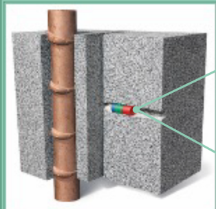
VPI580 corrosion inhibitor Margel™ is inserted into 20mm holes which are drilled in the concrete structure to be protected
